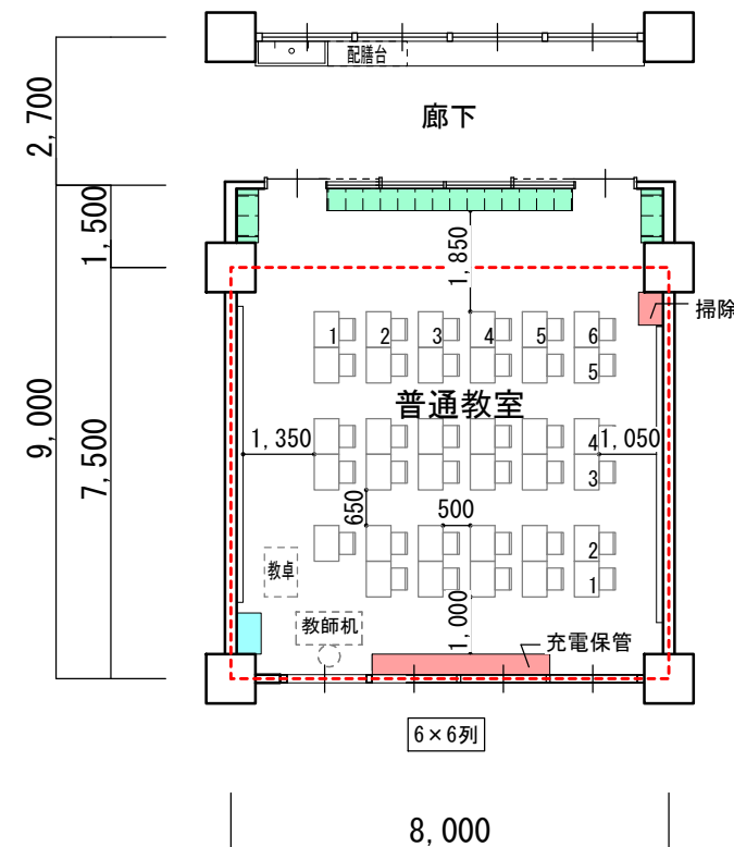
③ 72m 2 (8×9)
